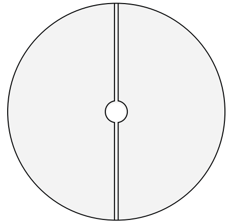
2-PIECE LID WITH 2" UMBRELLA HOLE
